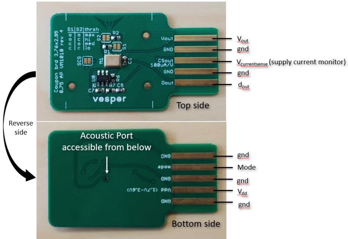
Figure 1. VM1010 Coupon PCB (Edge Connector recommendation is provided below)
